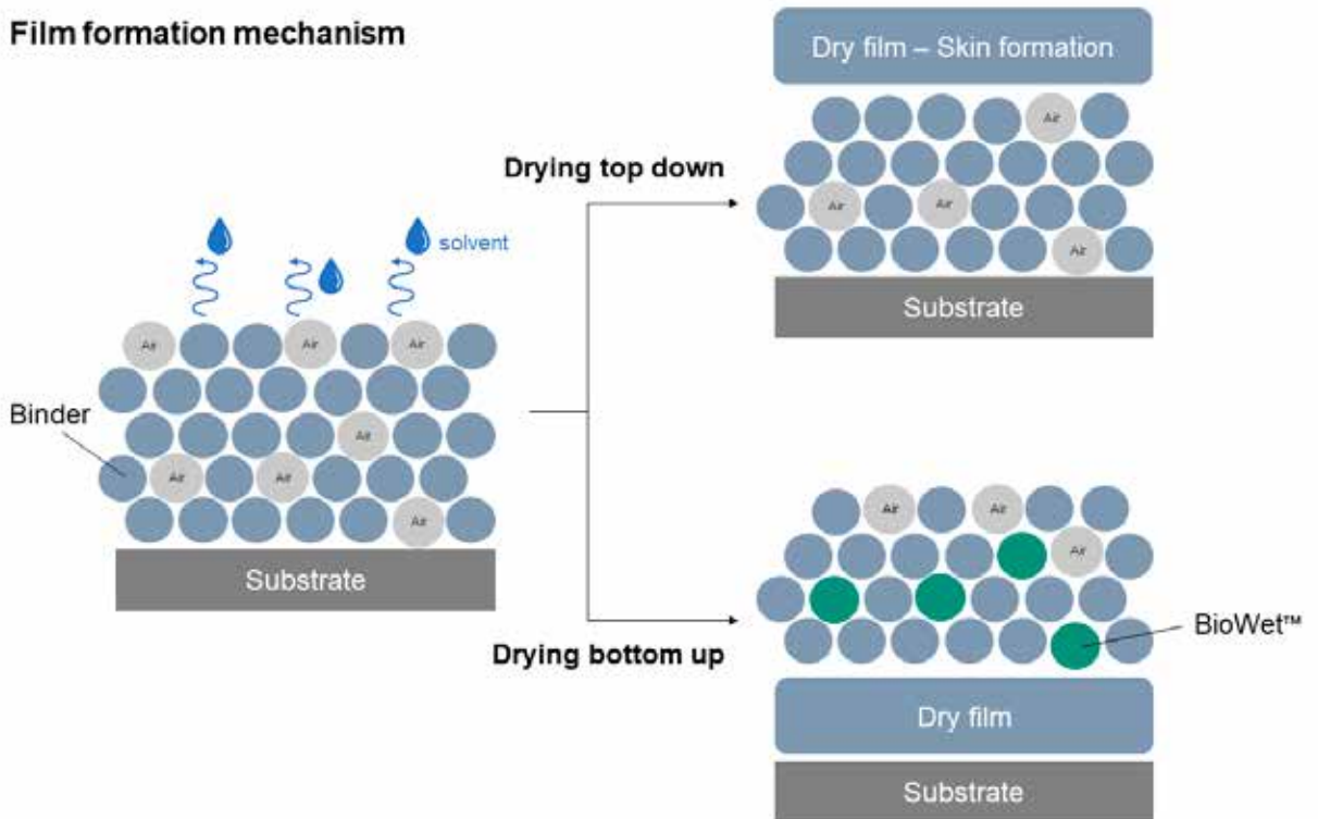
Schematic drying mechanism of BioFlow™/BioWet™ showing humectant properties.
